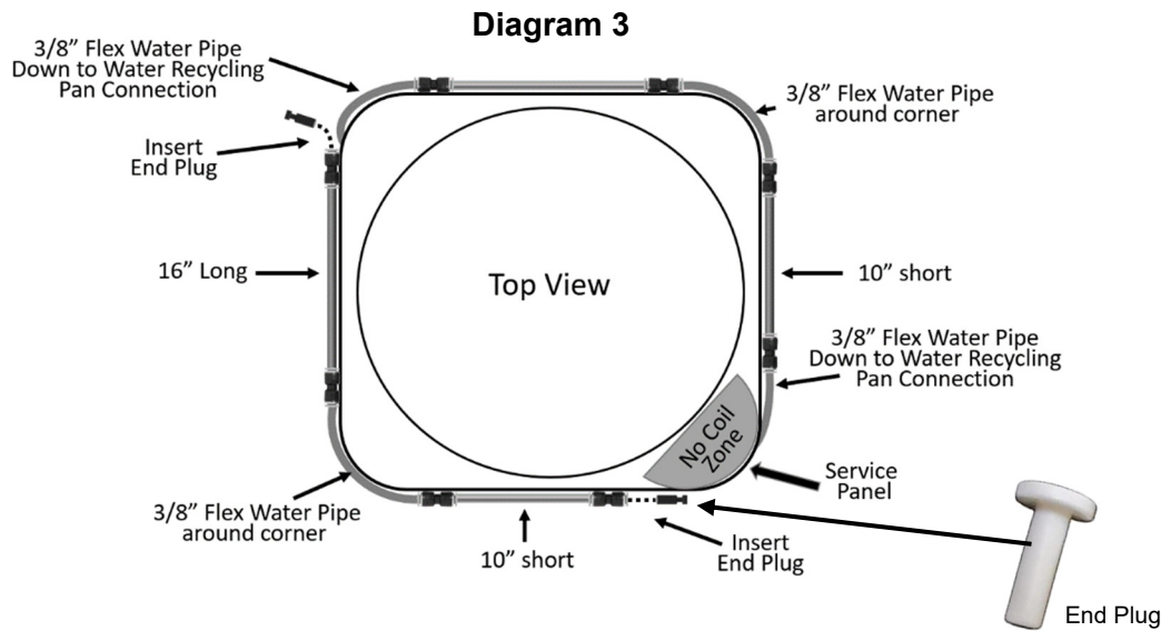
Condenser Type-1
